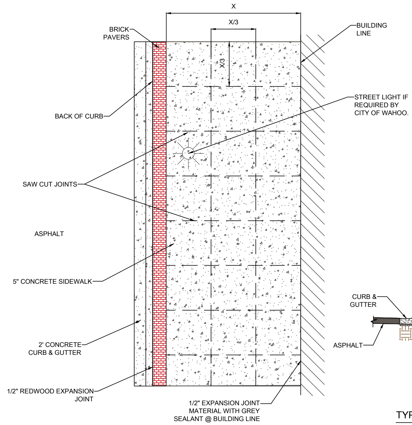
TYPICAL JOINT PATTERN
