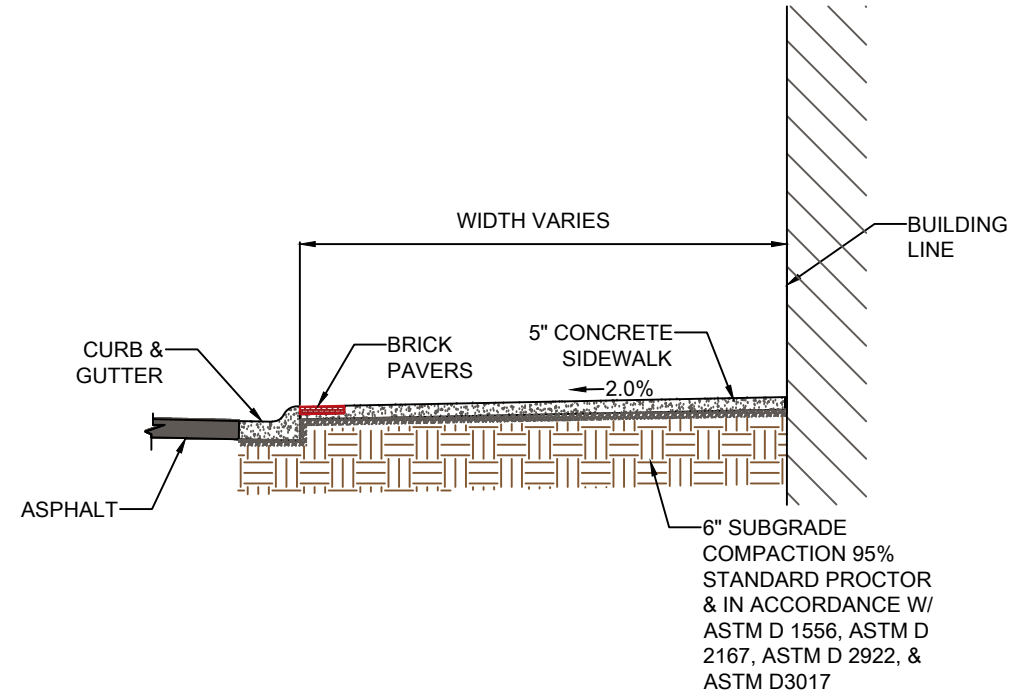
TYPICAL SIDEWALK CROSS SECTION
